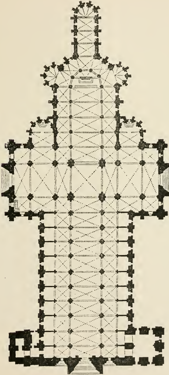
Fig. 300.—Notre-Dame, Rouen, ogival style. (Thirteenth Century.)
